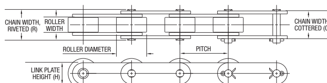
Oversized Roller (C2XX2)
