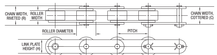
Oversized Roller Conveyor Series (C2XX2)
